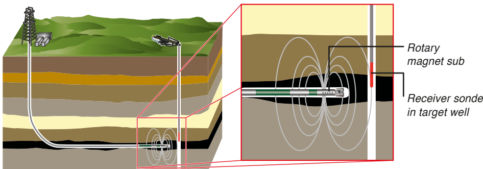
Figure 1-RMRS. A horizontal drill with the RMRS sub approaching a vertical hole containing the steering tool for magnetic ranging.
