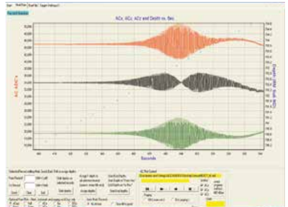
Shown are 3-component magnetic data from the rotating magnet sub. These data are analyzed for range and azimuth information for a single "shot."
